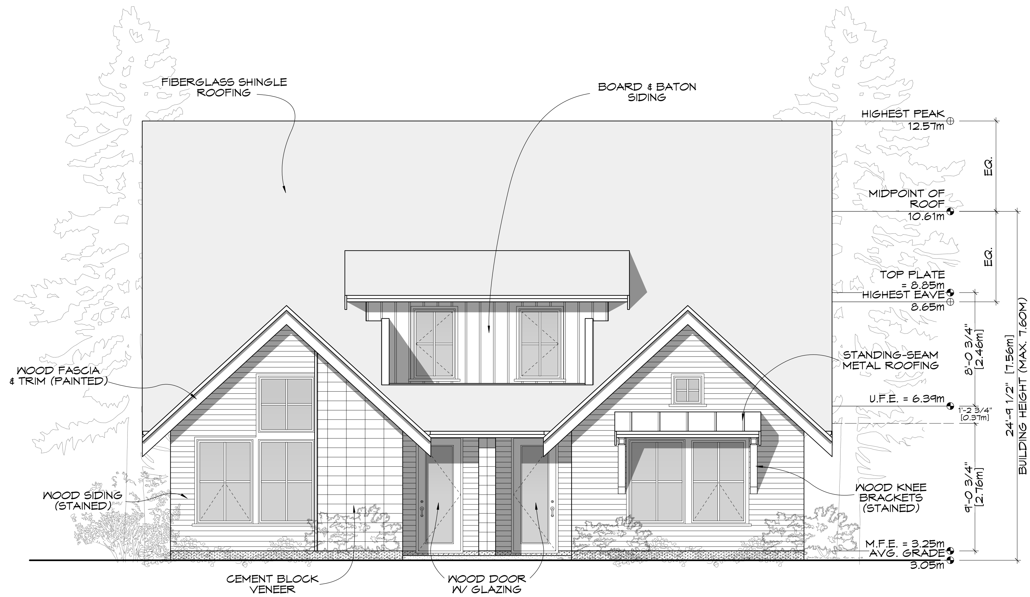
○ Front (N) Elevation Scale: 1/4" = 1'-0"
